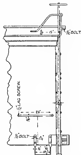
Fig. 5547. Side Elevation of Car End. RECOMMENDED PRACTICE FOR THE PROTECTION OF TRAINMEN.
